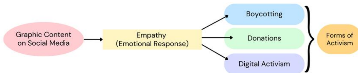
Figure 4. How Empathy Leads to Activism
